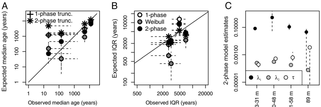
FIGURE 9. A, B, Comparison of median ages and interquartile ranges (IQR) observed in death assemblages and those predicted by five models of loss. In the three shallowest assemblages (from 23 to 58 m), both summary statistics are accurately predicted by a two-phase model (black circles): these predicted values lie closest to or on top of the diagonal line indicating equivalence with observed values. In contrast, the deepest assemblage (89 m; with median = 12,113 years and IQR = 4880 years) is best predicted by truncated-normal models (crosses and stars), indicating that production has not been constant. Some results plot on top of others so that not all 20 data points are visible. C, Estimates of loss rates \lambda_1 and \lambda_2 (black and gray circles, respectively) and of sequestration rate \tau (white circles) for AFDs along a bathymetric gradient (with bootstrapped 95% confidence intervals). Even though the shapes of AFDs change markedly with increasing water depth (x-axis), each parameter remains fairly constant along the bathymetric gradient, with \lambda_1 and \lambda_2 differing consistently by two orders of magnitude.
